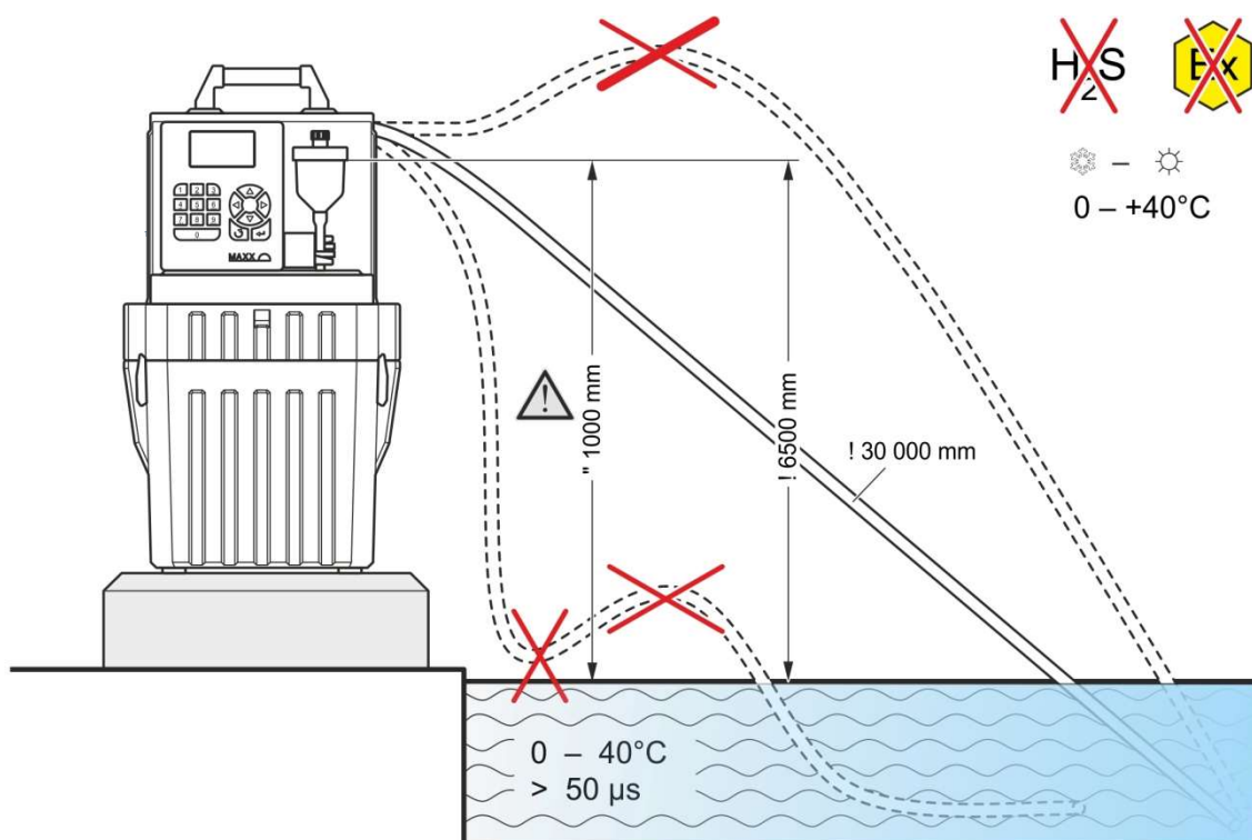
Figure 18 Installation diagram
