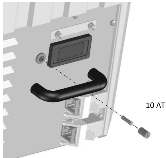
Figure 51 Position of the fuse in the optional bottle compartment with active cooling
