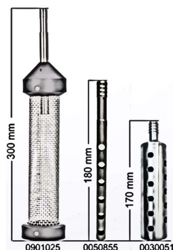
Figure 57 Strainers
