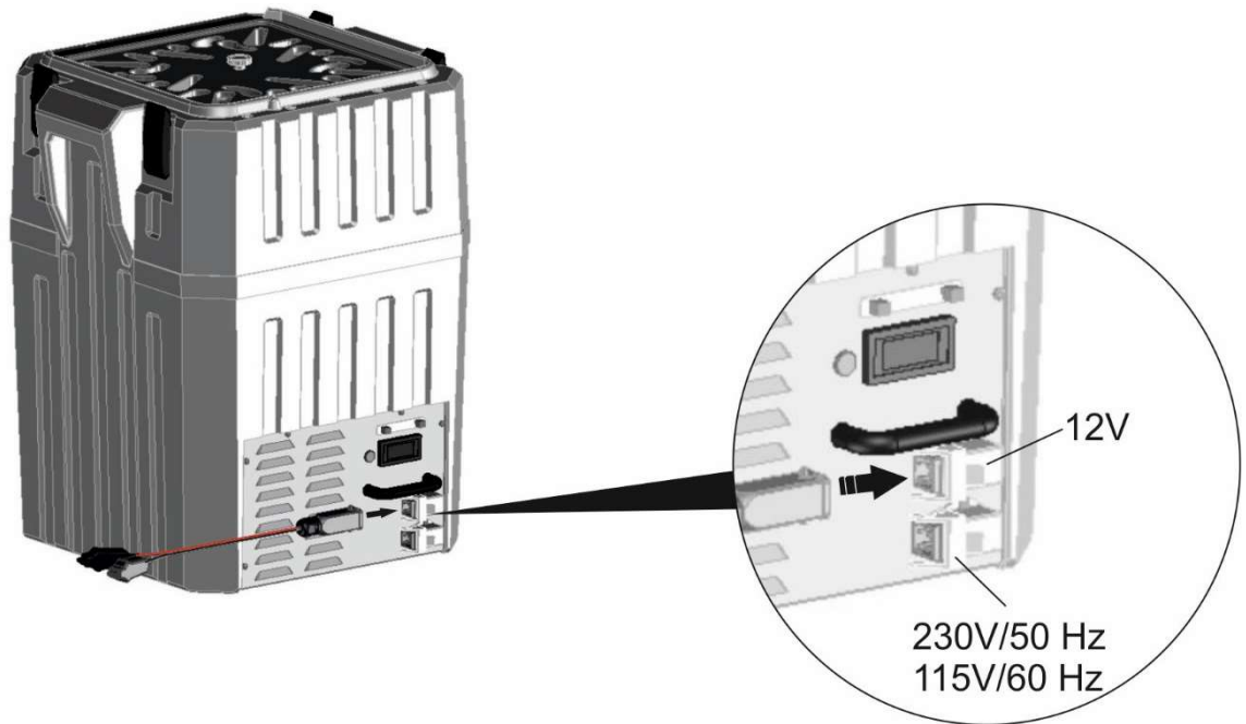
Figure 37 Potential connection variations (optional bottle compartment with active cooling)
