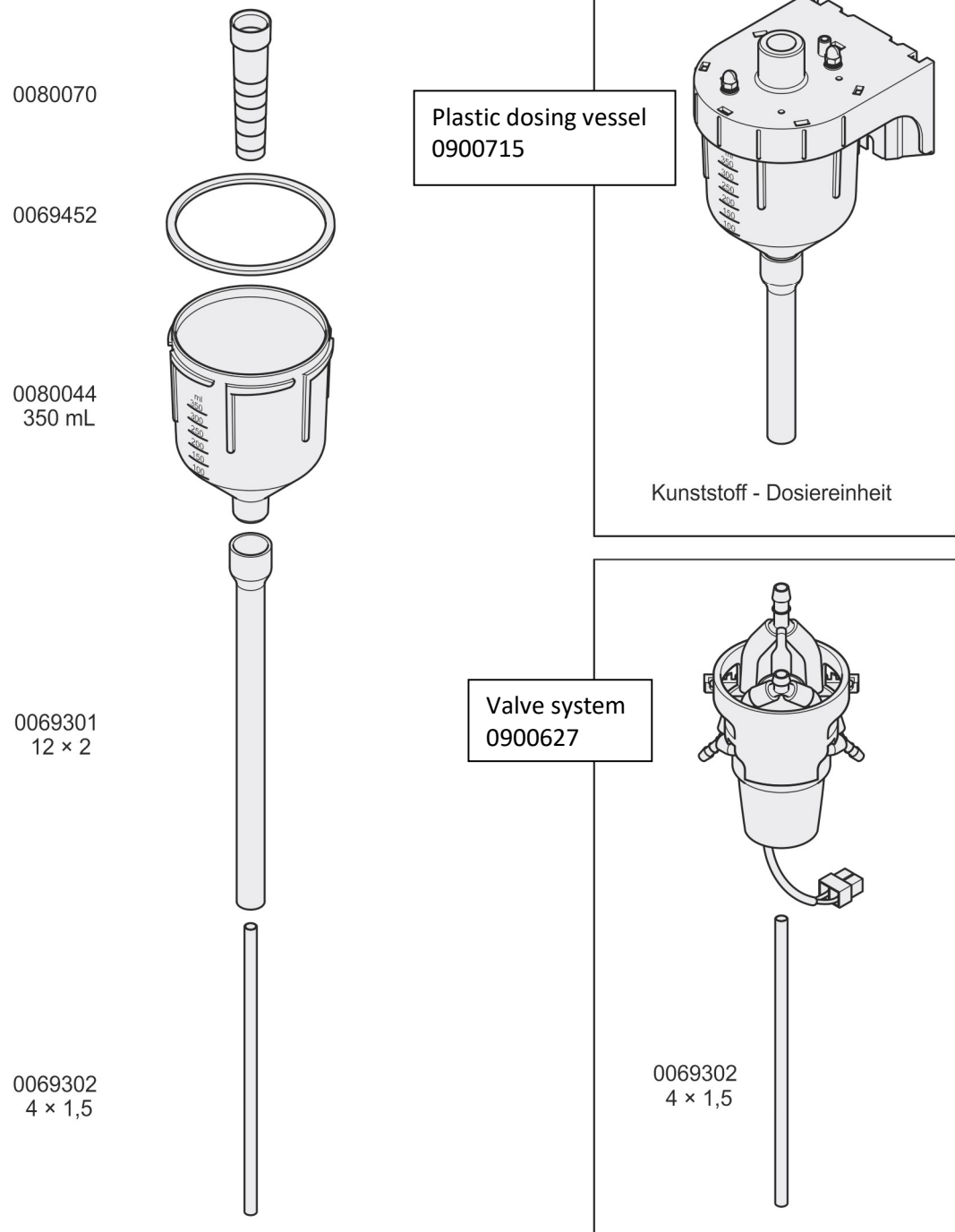
Figure 52 Plastic dosing vessel
