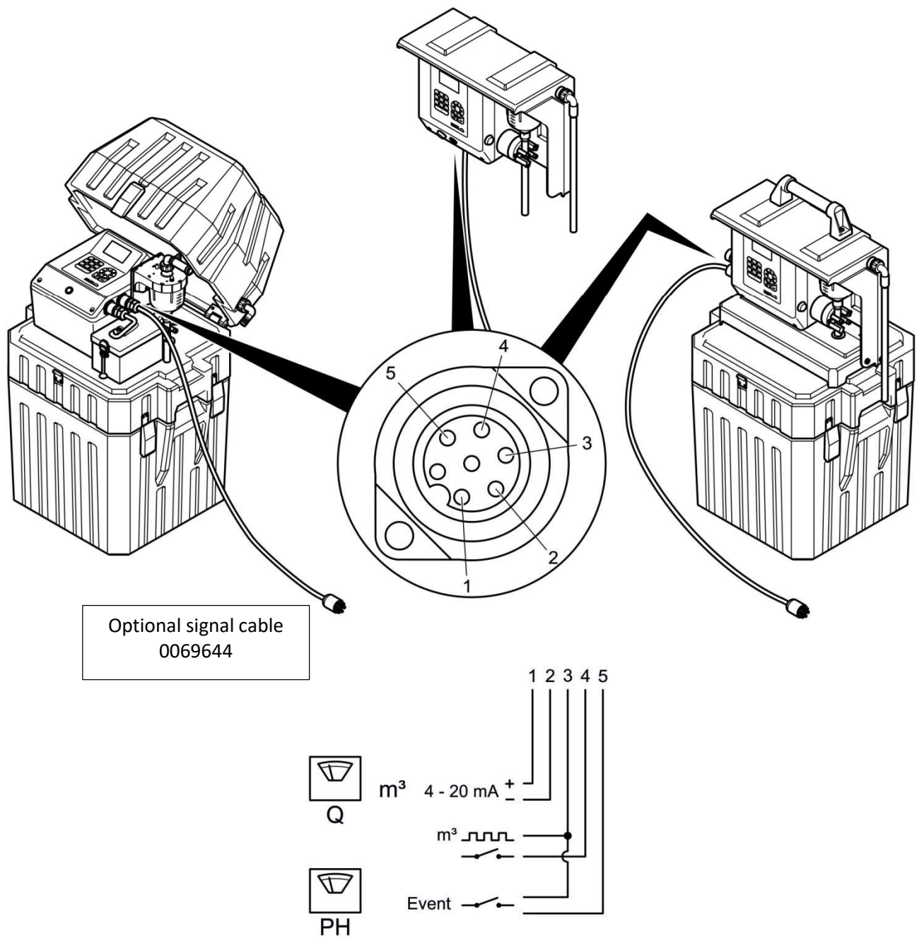
Figure 13 Connection plan for the optional signal cable (0069644)
