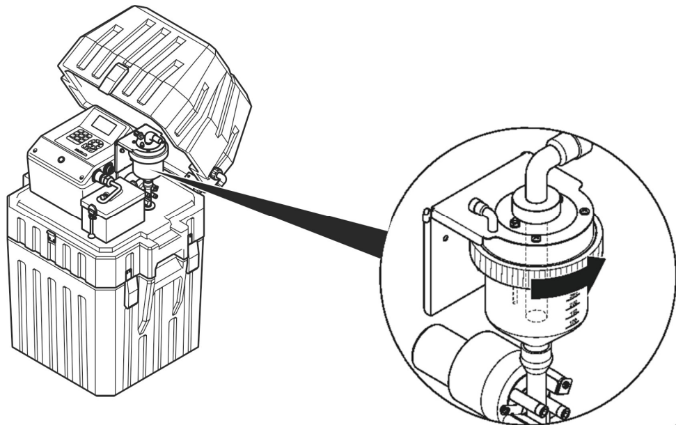
Figure 26 Assemble the glass dosing vessel
