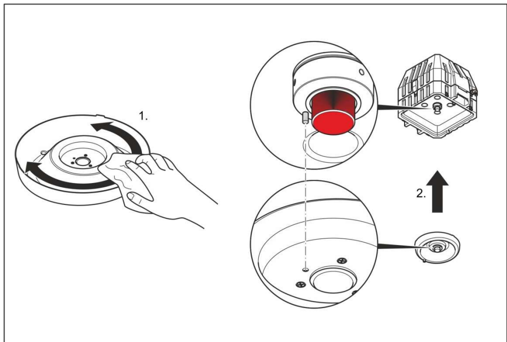
Figure 44 Assemble the distribution vat (TP5 P und TP5 C)
